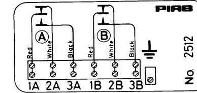
Two microswitches
