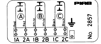
Three microswitches
