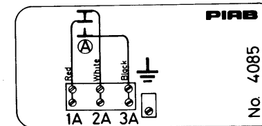
One microswitch
